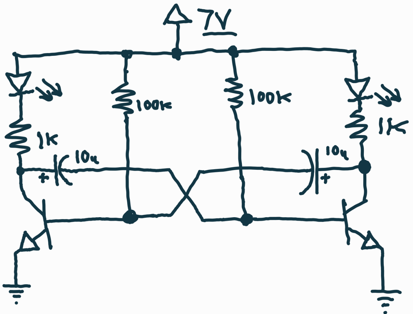
ASTABLE MULTIVIBRATOR
