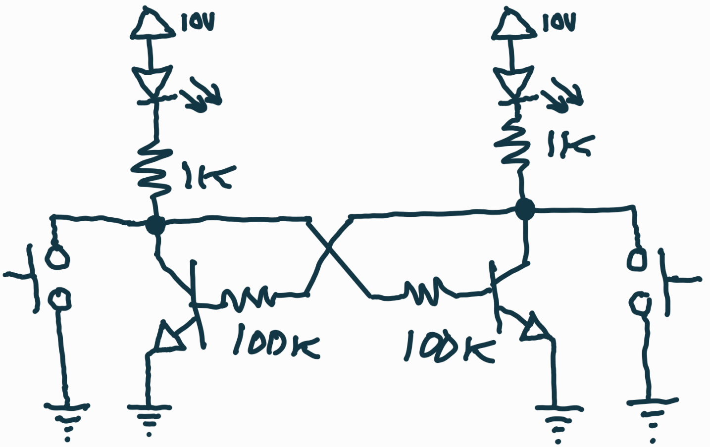
SIMPLE FLIP-FLOP.
