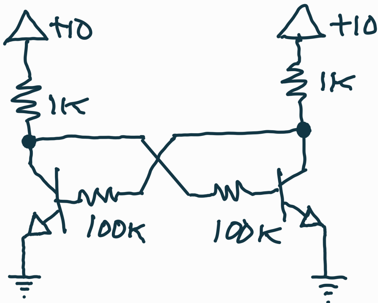
CROSS-COUPLED PAIR
