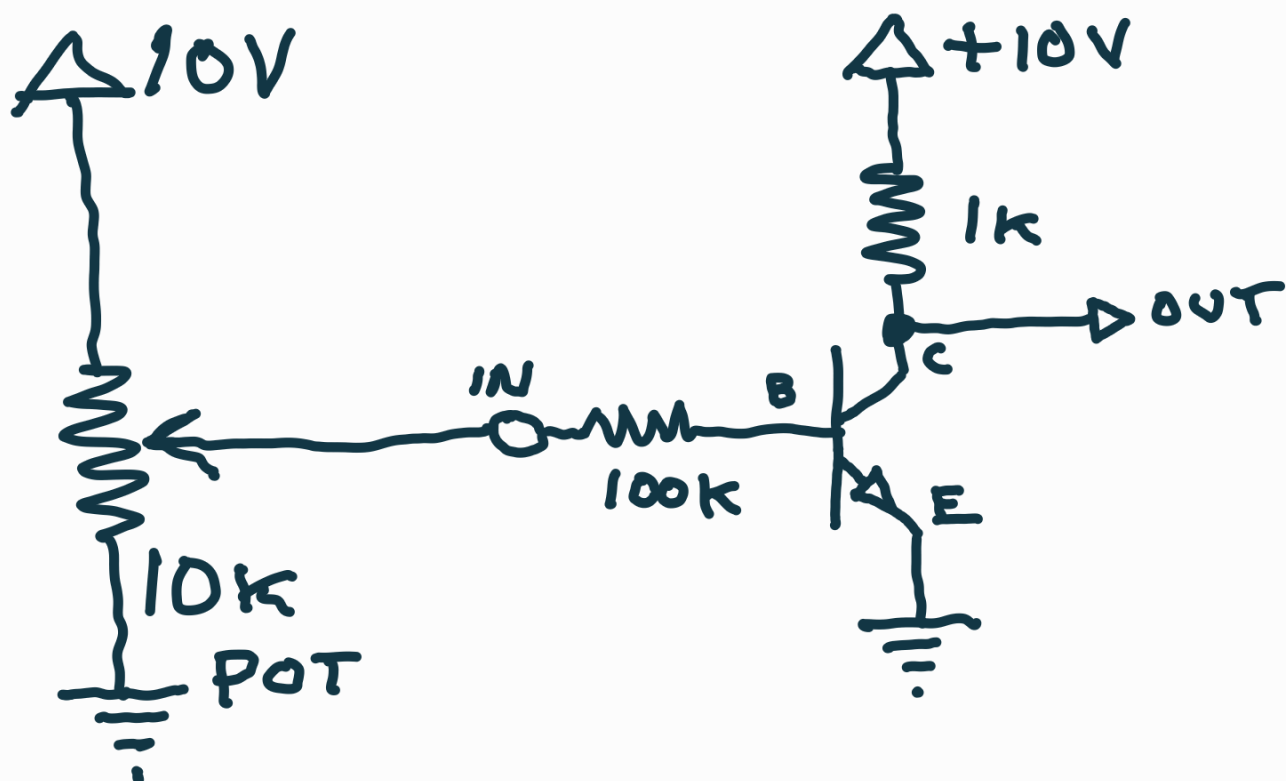
ANALOG INVERTER
