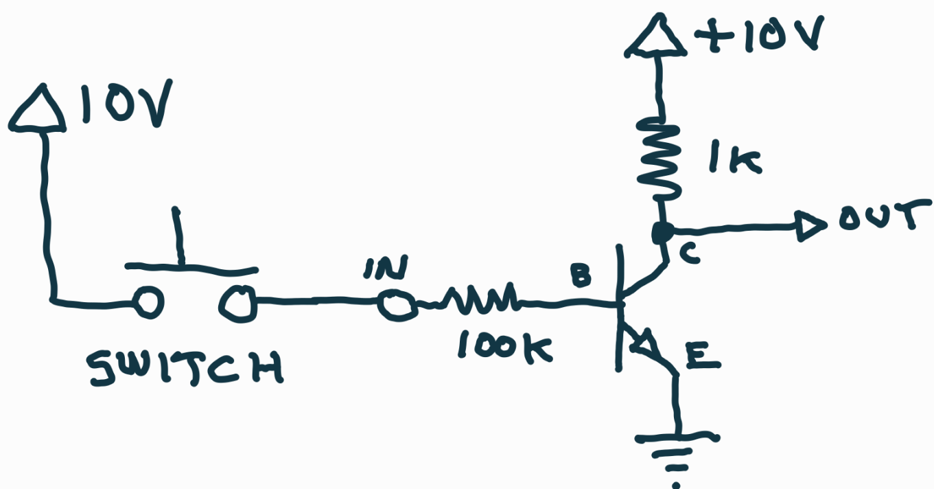
DIGITAL INVERTER.
